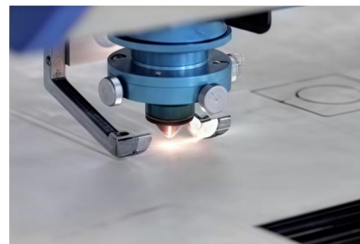
激光头 Laser Head
